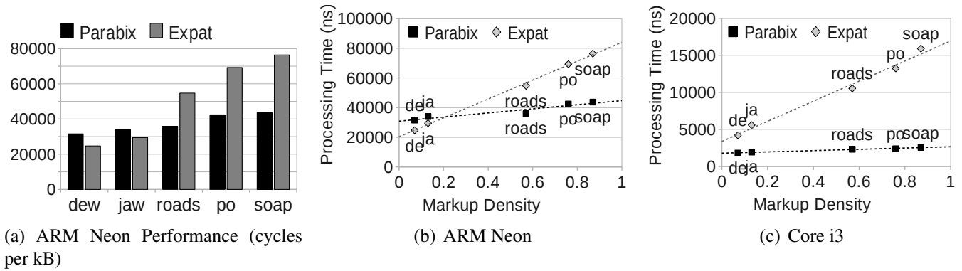
1145 Figure 15: Comparison of Parabix-XML on ARM vs. Intel.
