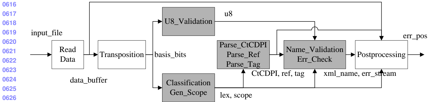
Figure 7: Parabix XML Parser Structure
