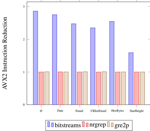
Figure 10: Instruction Reduction
