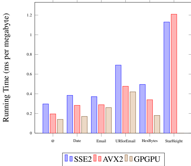
Figure 12: Running Time
